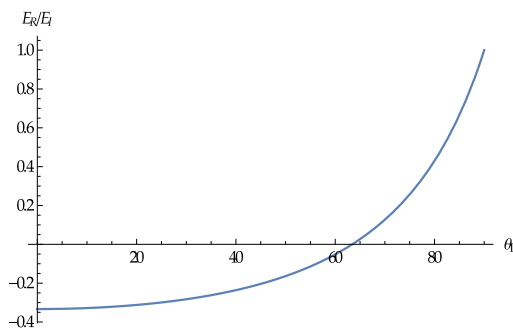
Figure 68: The reflected field with parallel polarisation
