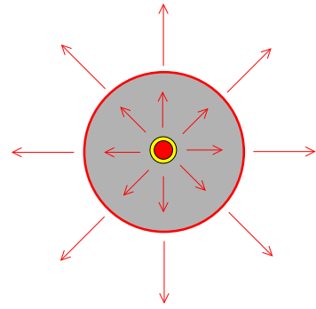
Figure 60: A polarised material
