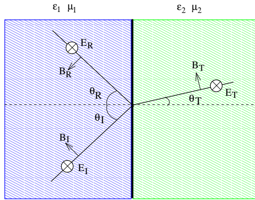
Figure 64: Incident, reflected and transmitted waves with normal polarisation.
