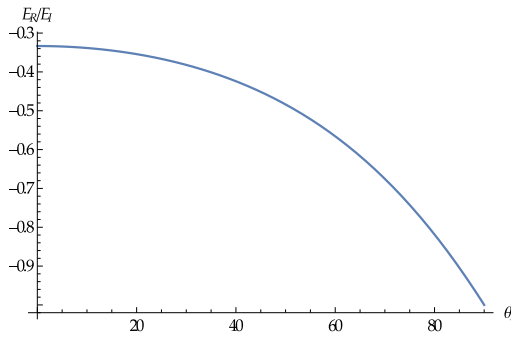
Figure 65: The reflected field with normal polarisation
