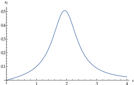
Figure 72: The imaginary part of the permittivity, \epsilon_2
