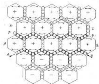
Figure 44: Maxwell's vortices
