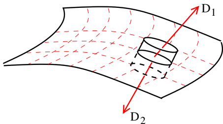
Figure 61: The normal component of the electric field is discontinuous
