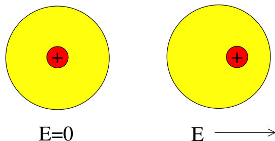
Figure 58: The polarisation of an atom
