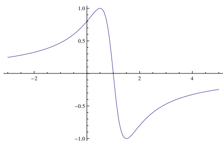
Figure 74: The real part of the function plotted with \omega' = 1 and \epsilon = 0.5 .
