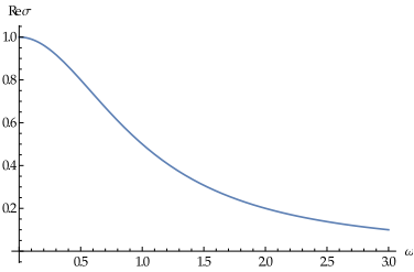
Figure 76: The real, dissipative part of the conductivity
