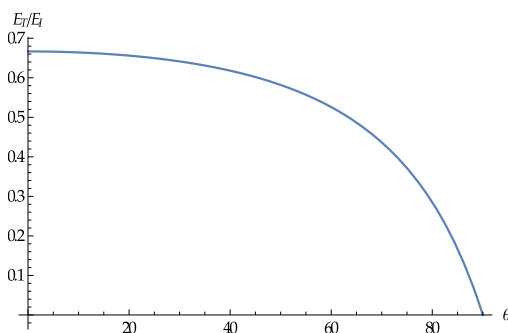
Figure 69: The transmitted field with parallel polarisation
