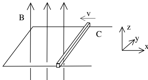
Figure 35: Moving circuit
