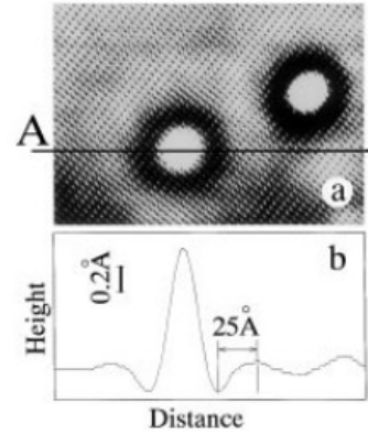
Figure 79: Friedel oscillations in GaAs doped with Silicon.
