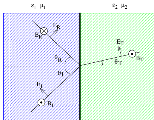
Figure 67: Incident, reflected and transmitted waves with parallel polarisation.
