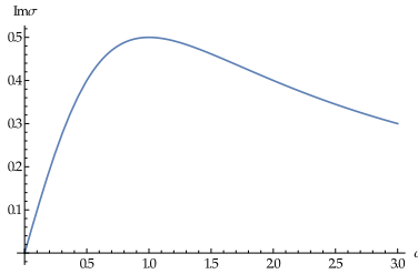
Figure 77: The imaginary, reactive part of the conductivity
