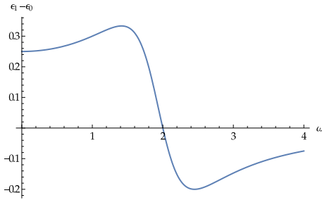
Figure 71: The real part of the permittivity, \epsilon_1 - \epsilon_0
