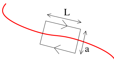
Figure 62: The tangential component of the electric field is continuous.
