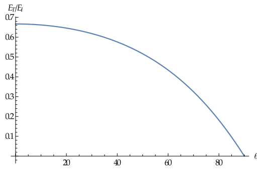
Figure 66: The transmitted field with normal polarisation
