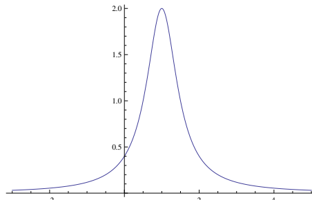
Figure 75: The imaginary part of the function plotted with \omega' = 1 and \epsilon = 0.5 .
